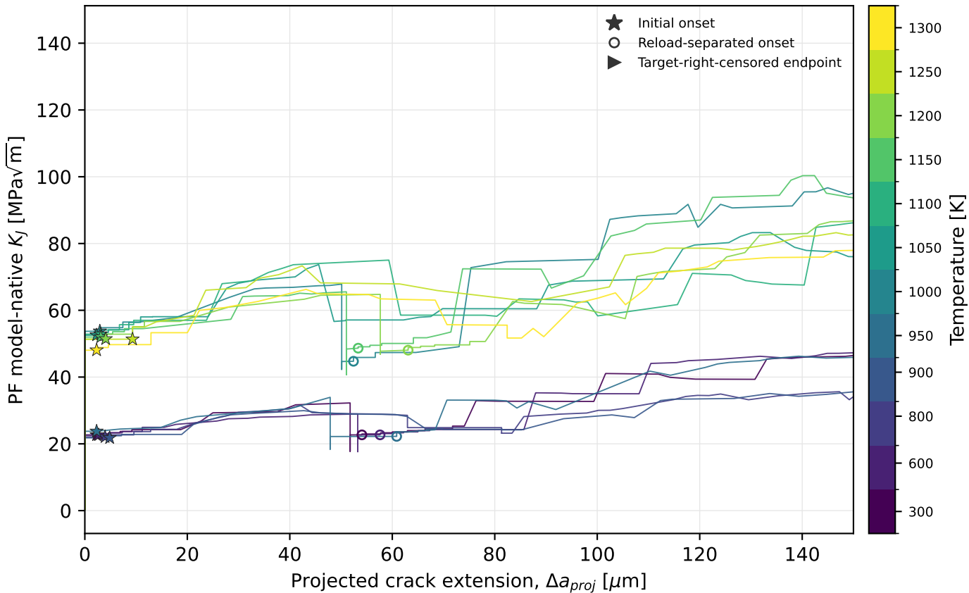
DBTT: theta=0 deg, rate0p01x PF MODEL-NATIVE KJ TRAJECTORY — EARLY RANGE
