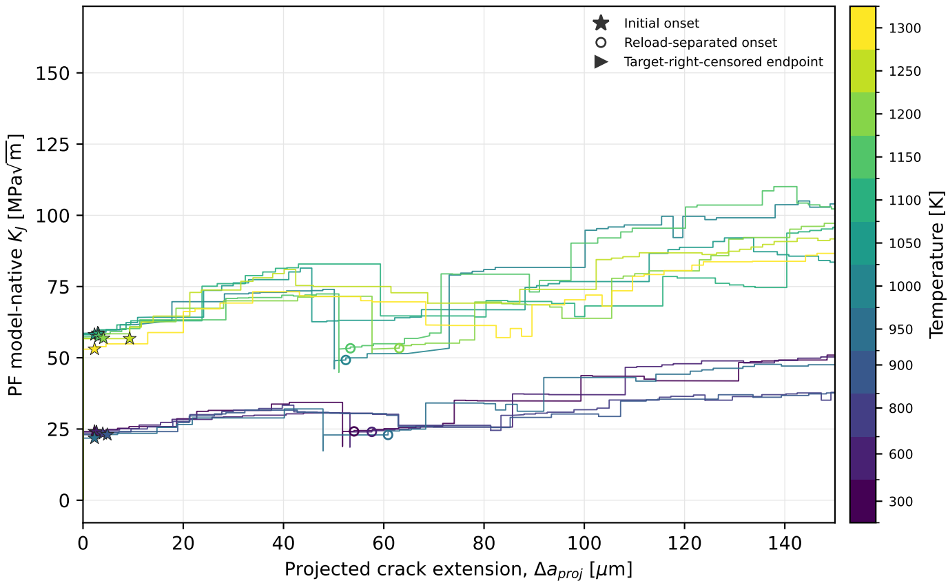
DBTT: theta=0 deg, rate100x PF MODEL-NATIVE K J TRAJECTORY — EARLY RANGE
