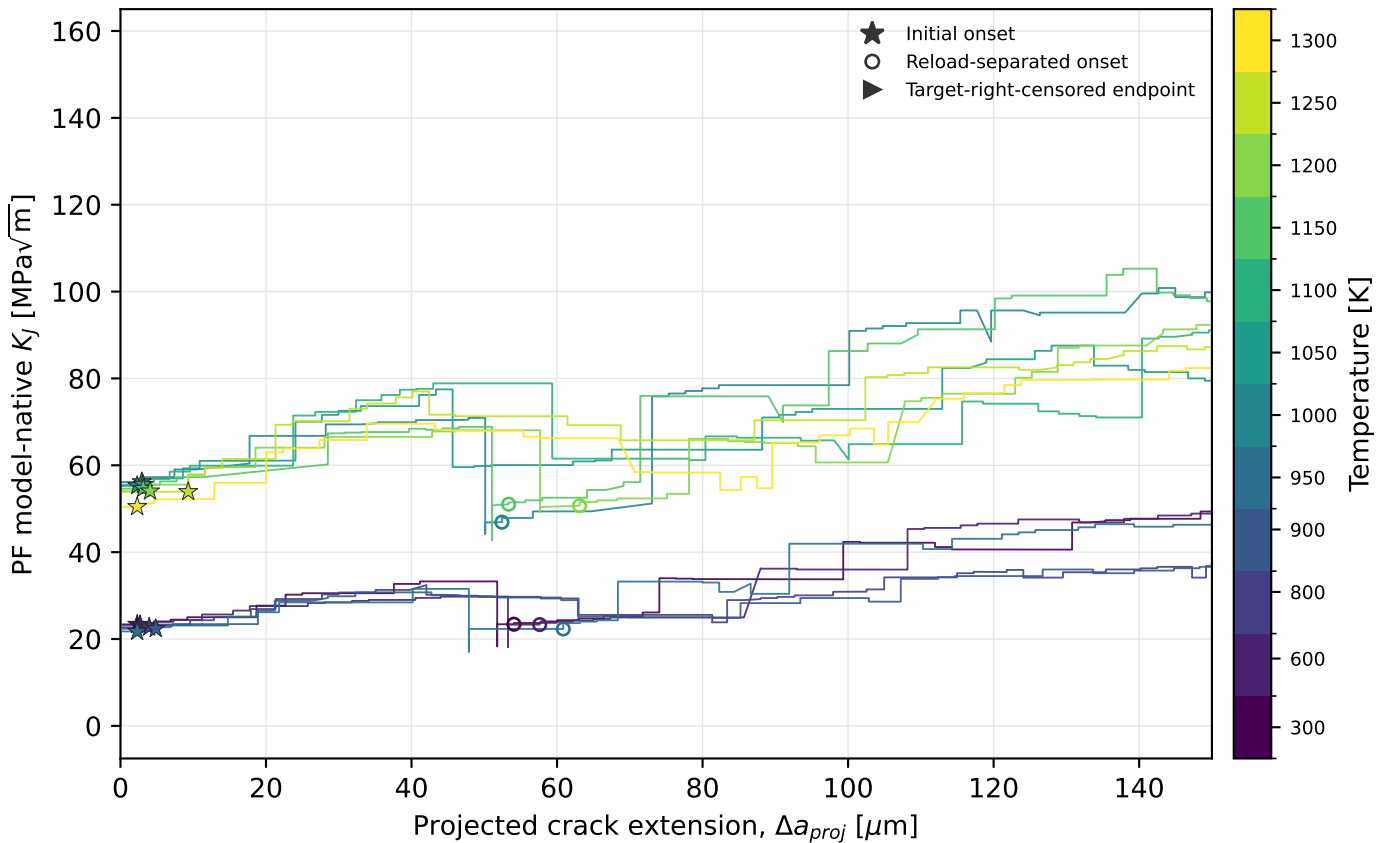
DBTT: theta=0 deg, rate1x PF MODEL-NATIVE K J TRAJECTORY — EARLY RANGE
