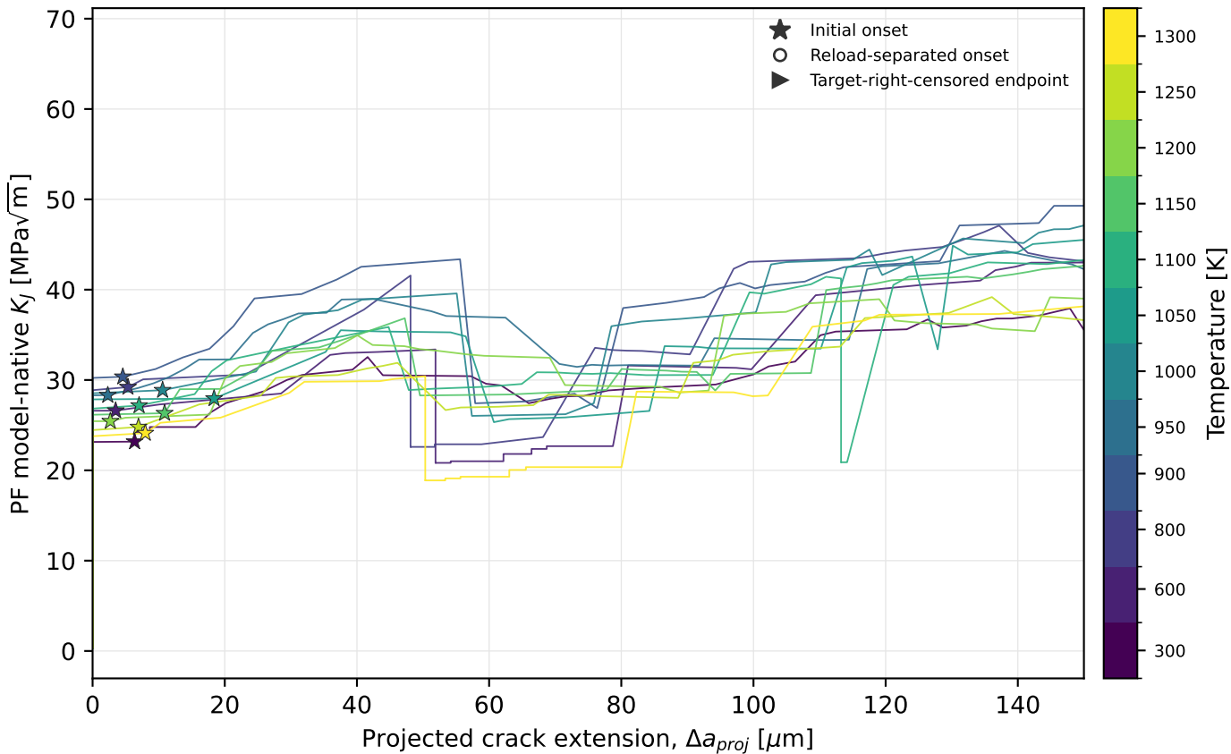
weak-T: \theta=0 deg, rate0p01x PF MODEL-NATIVE KJ TRAJECTORY — EARLY RANGE
