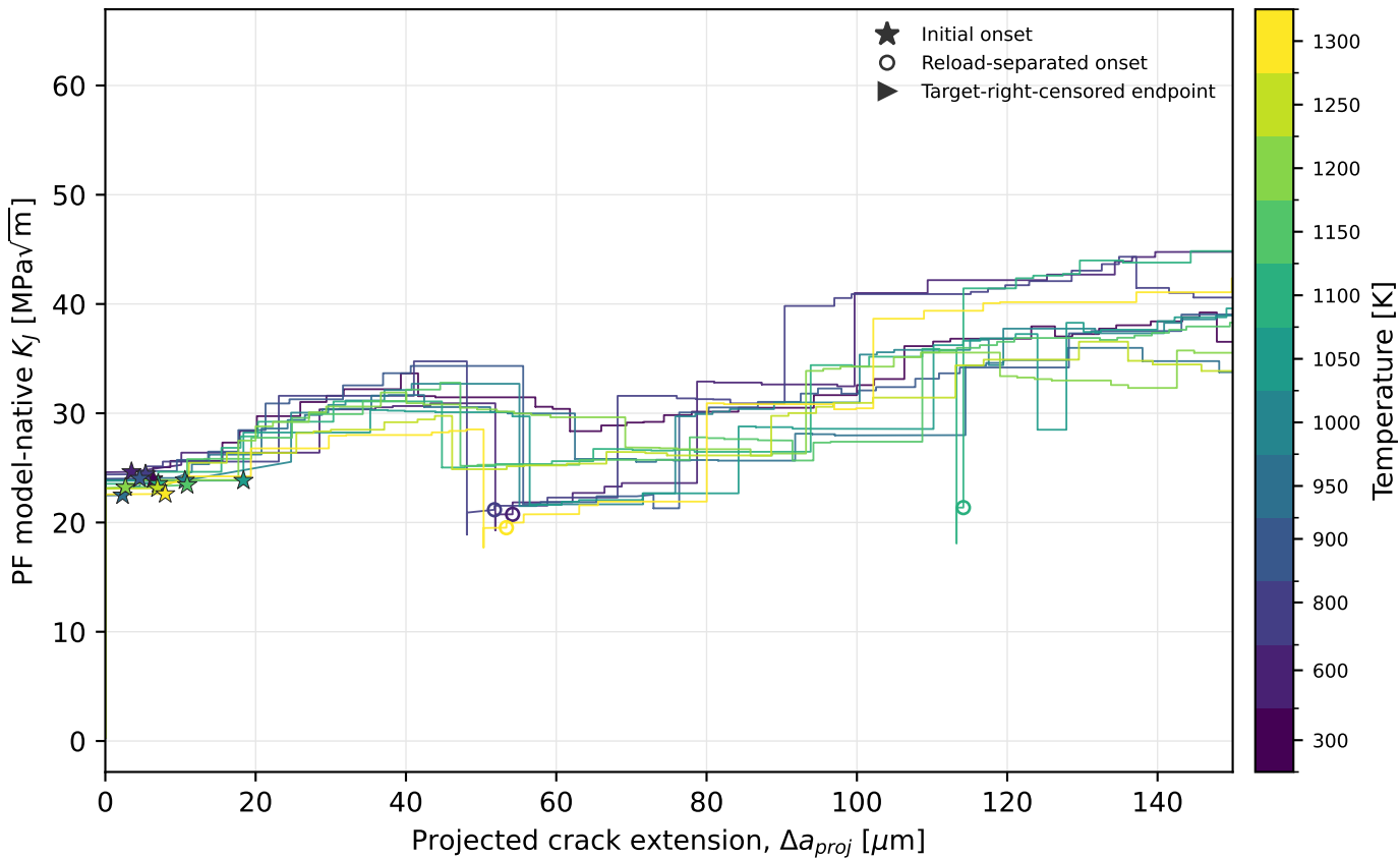
weak-T: theta=0 deg, rate100x PF MODEL-NATIVE KJ TRAJECTORY — EARLY RANGE
