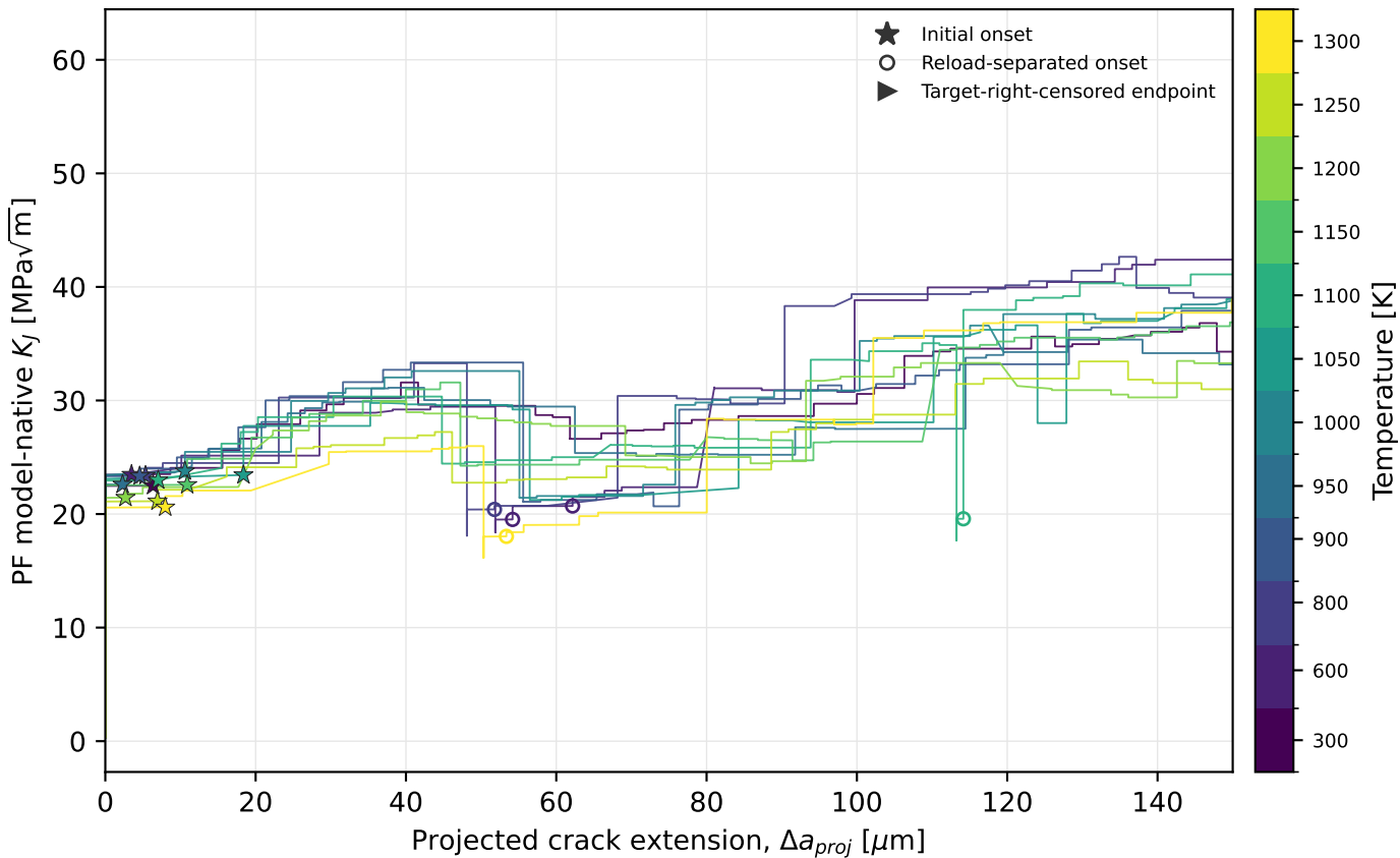
weak-T: theta=0 deg, rate1x PF MODEL-NATIVE KJ TRAJECTORY — EARLY RANGE
