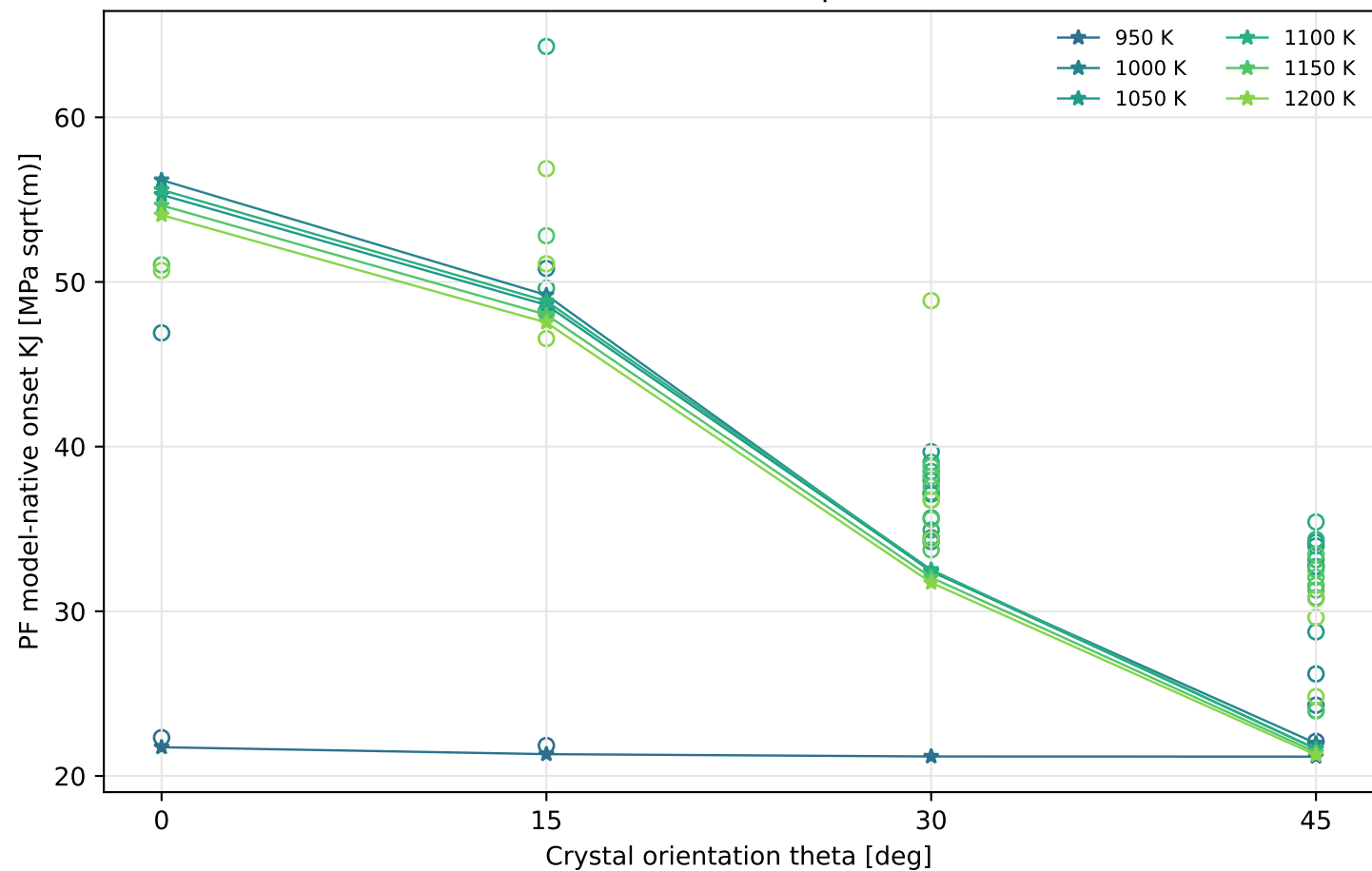
DBTT: initial stars and reload-separated onset circles
