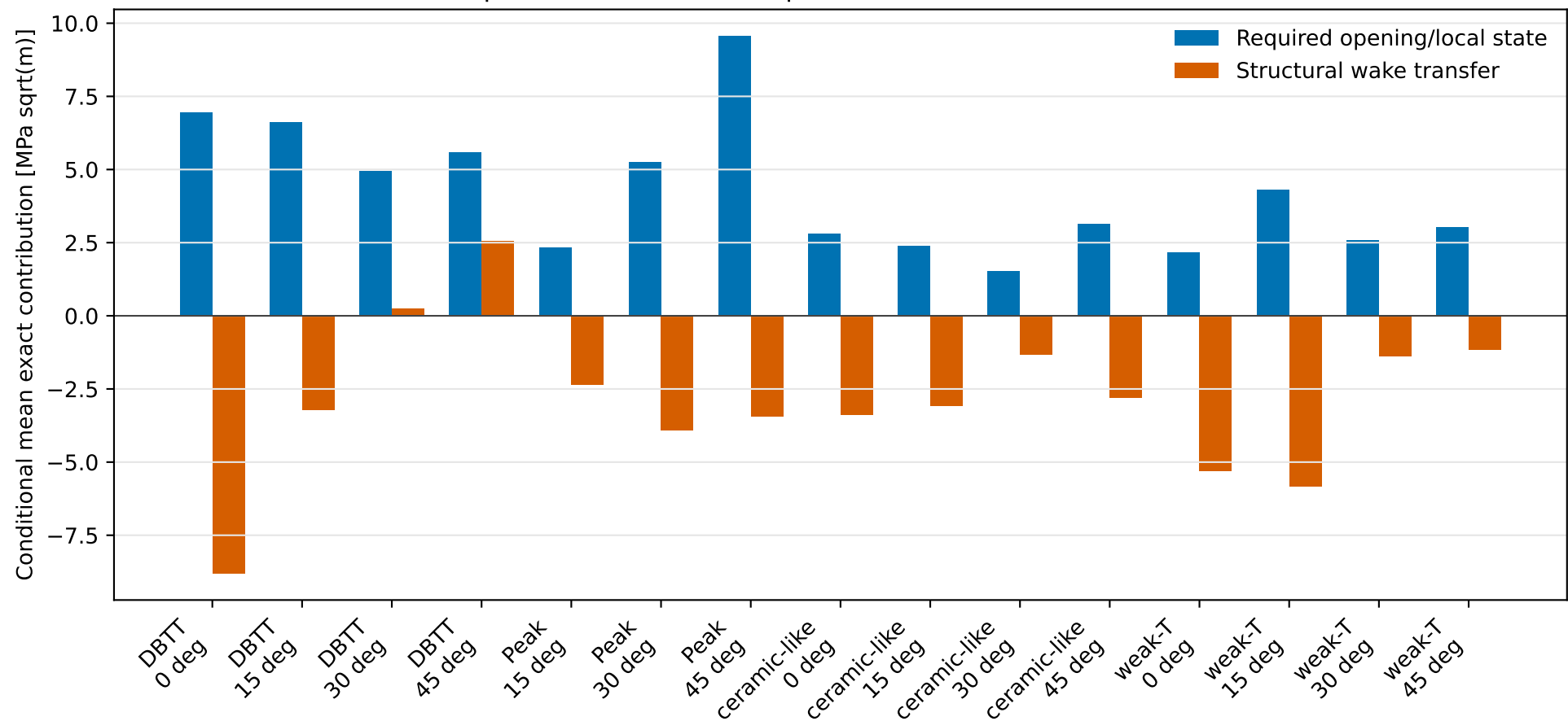
Reload-separated Delta K decomposition (conditional on finite reinitiation)
