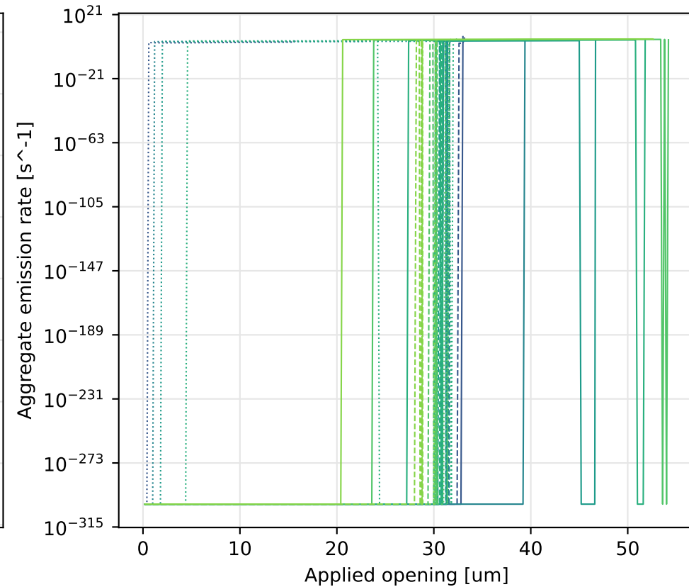
Peak theta=0 deg cleavage/emission competition (900-1200 K)
