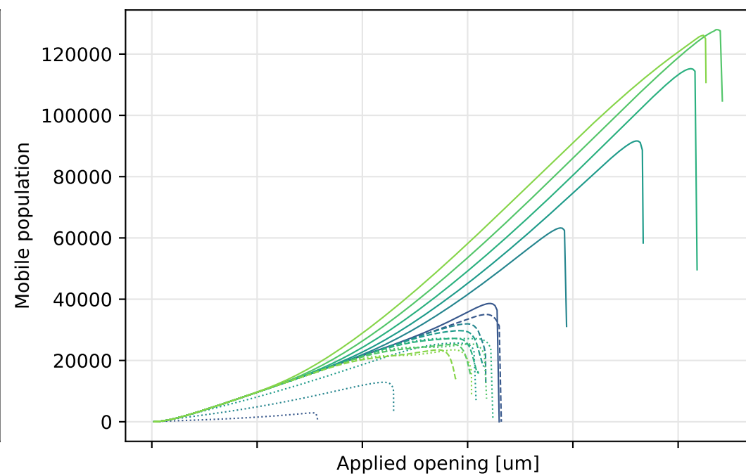
Peak theta=0 deg pre-initiation state versus opening (900-1200 K)
