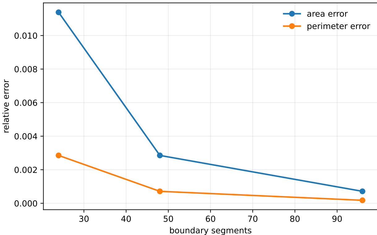
VOIDING V1 CIRCULAR HOLE KIRSCH BENCHMARK
