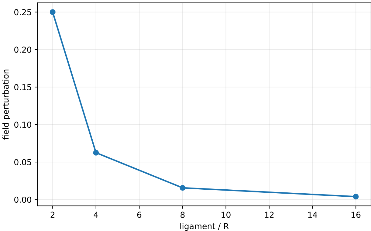
VOIDING V1 CRACK TIP FIELD VS VOID DISTANCE
