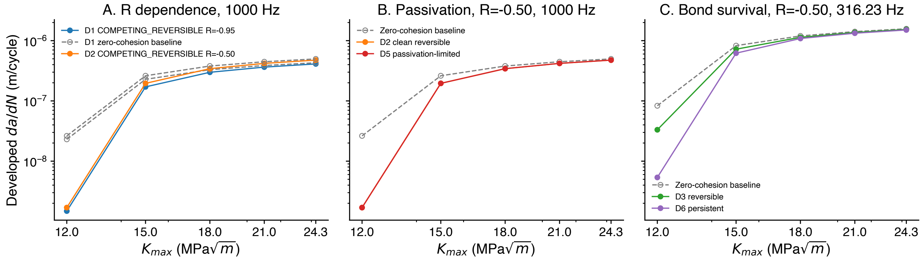
Figure 3. Crack-rebonding parameterizations (PX4 developed points, signed-K contact surrogate -- opposing crack-face contact is not resolved)
