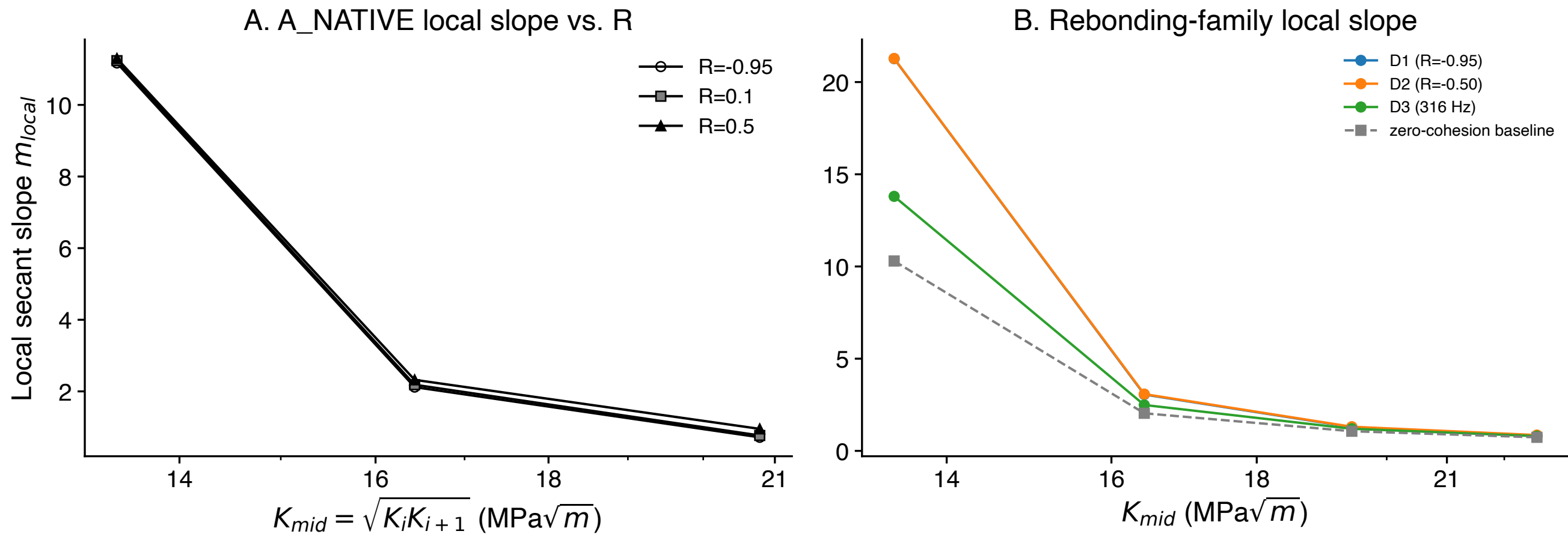
Figure 4. Local (adjacent-secant) slopes -- primary local-slope measure
