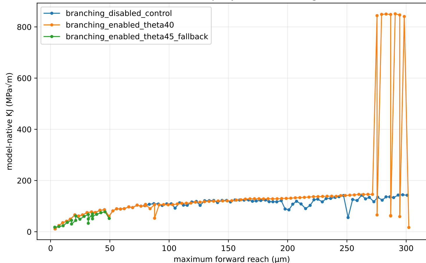
PF model-native directional KJ trajectories (not toughness/R-curve)
