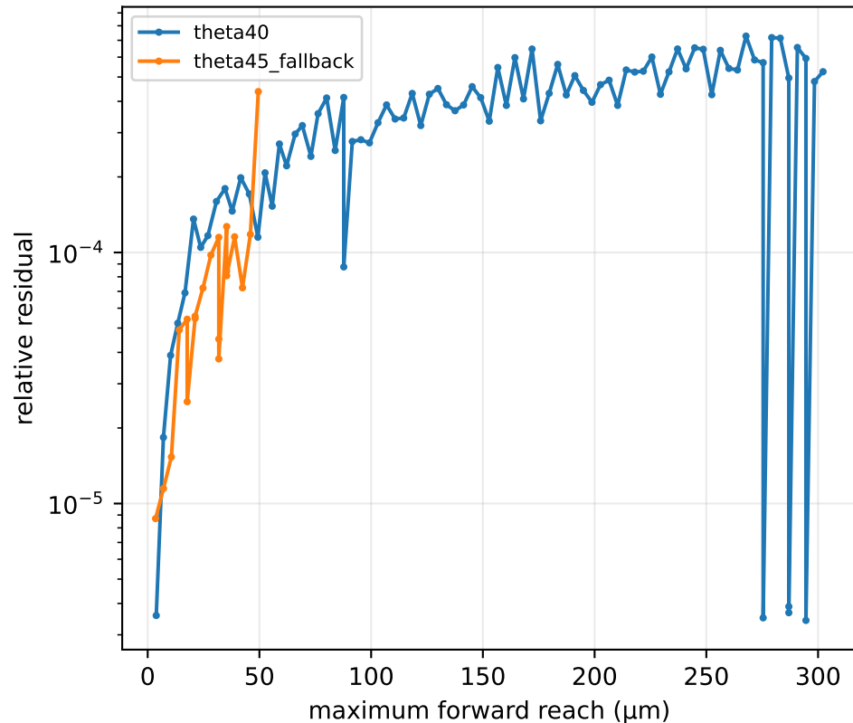
Accepted atomic-action energy residual
