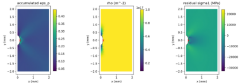
Shielded (seed 5, 900 MPa) (no verified common field normalization)
