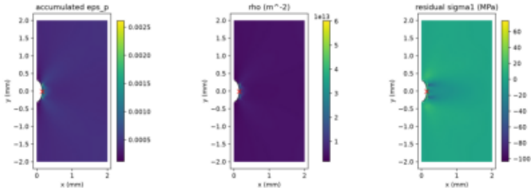
Unshielded (seed 5, 900 MPa)
