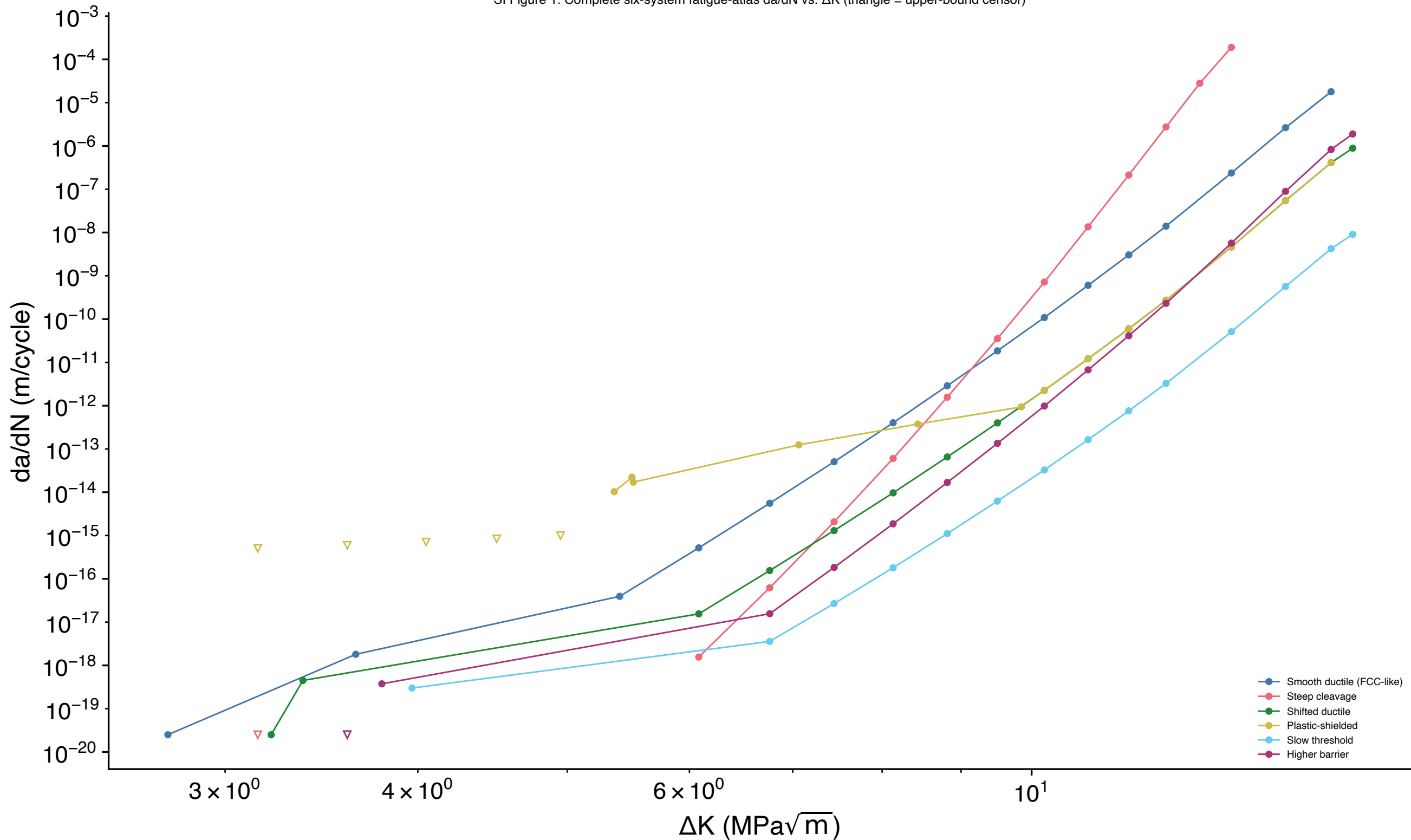
SI Figure 1. Complete six-system fatigue-atlas da/dN vs. \Delta K (triangle = upper-bound censor)
