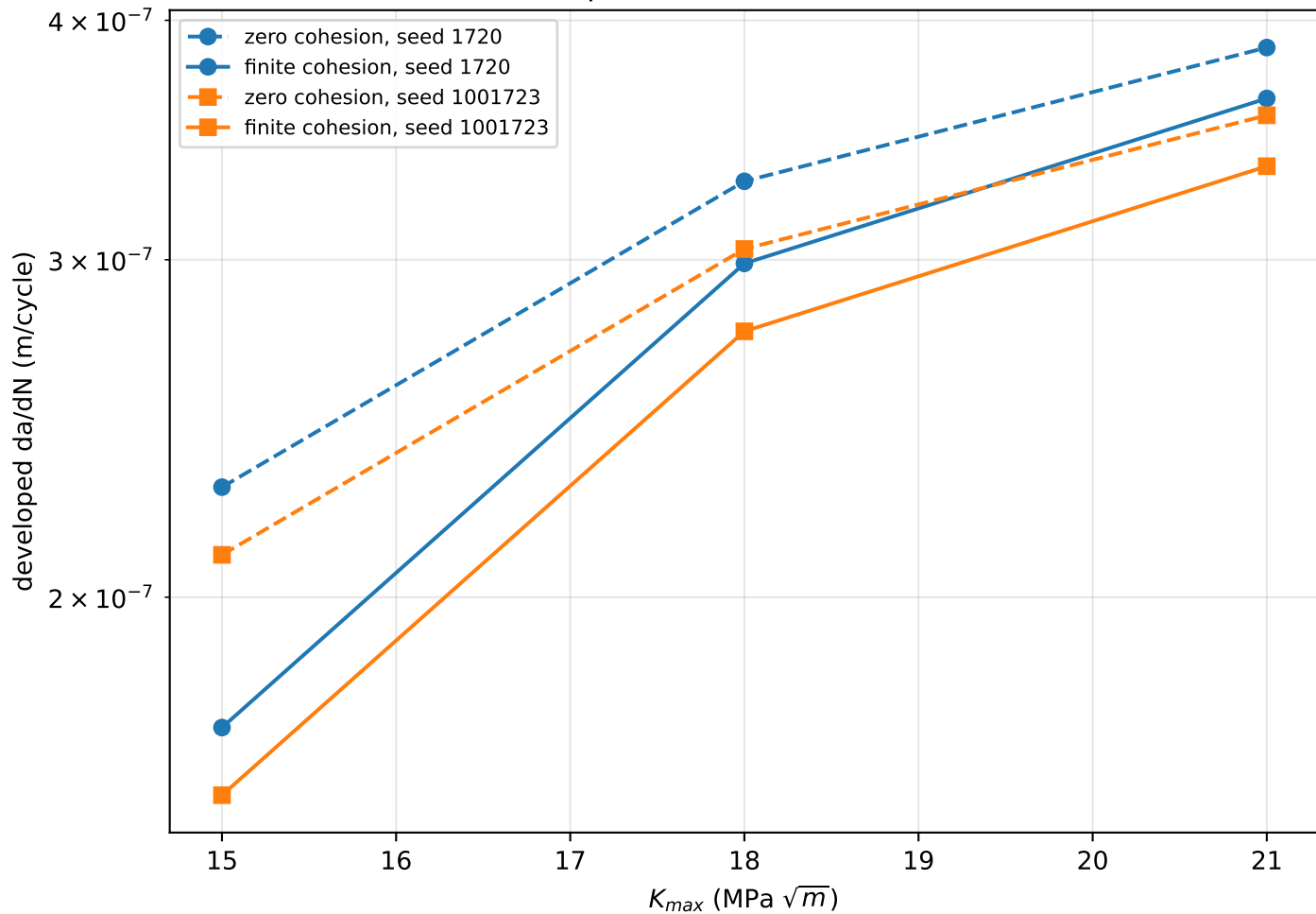
Developed-window da/dN vs Kmax
