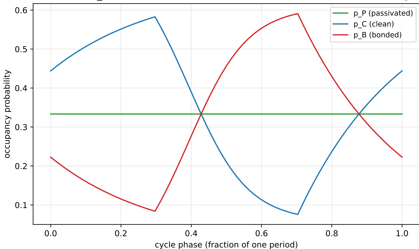
ANALYTICAL PREDICTION: P/C/B periodic-orbit phase trajectory COMPETING_REVERSIBLE, K_{\max}=18 \text{ MPa}\sqrt{m} , R=-0.5 , f=1000\text{Hz} (zero fitting)
