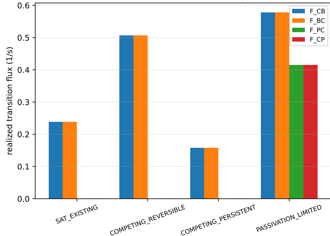
Realized transition fluxes (analytical)
