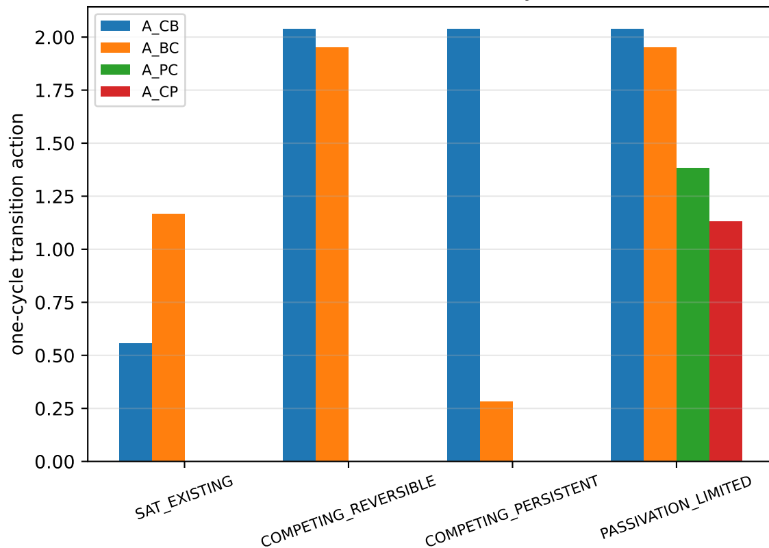
Transition actions (analytical)
