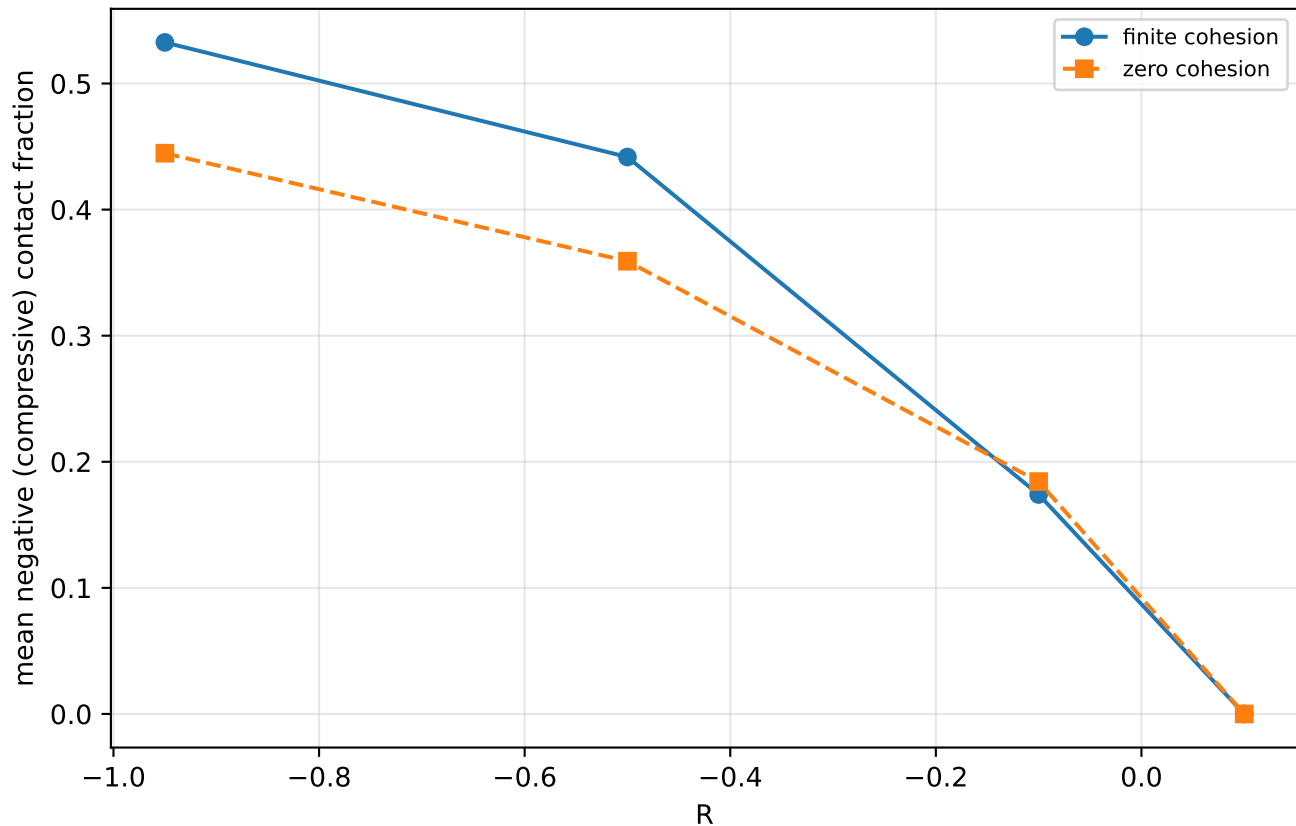
PHYSICAL SIMULATION: PX3 screen contact-exposure fraction vs R (Kmax=18 MPa \sqrt{m} , f=1000Hz reference)
