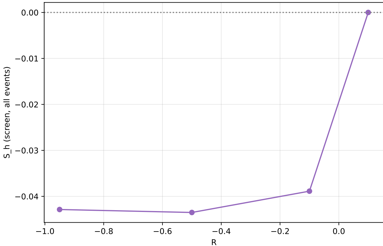
PHYSICAL SIMULATION (POST-PROCESSED): PX3 screen S_h vs R ( K_{\max}=18 \text{ MPa}\sqrt{m} , f=1000\text{Hz} reference)
