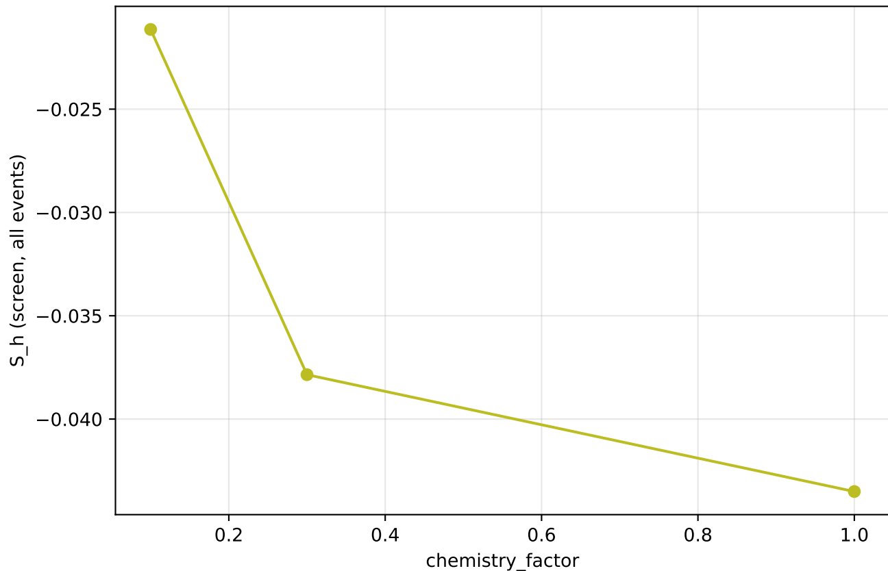
PHYSICAL SIMULATION (POST-PROCESSED): PX3 screen passivation/chemistry response (PASSIVATION_LIMITED row, Kmax=18 MPa \sqrt{m} reference)
