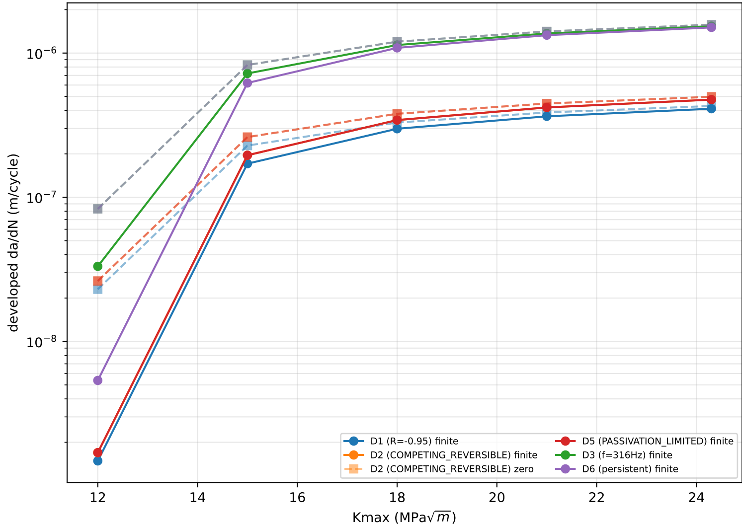
PHYSICAL SIMULATION: absolute developed da/dN vs Kmax, seed=1720
