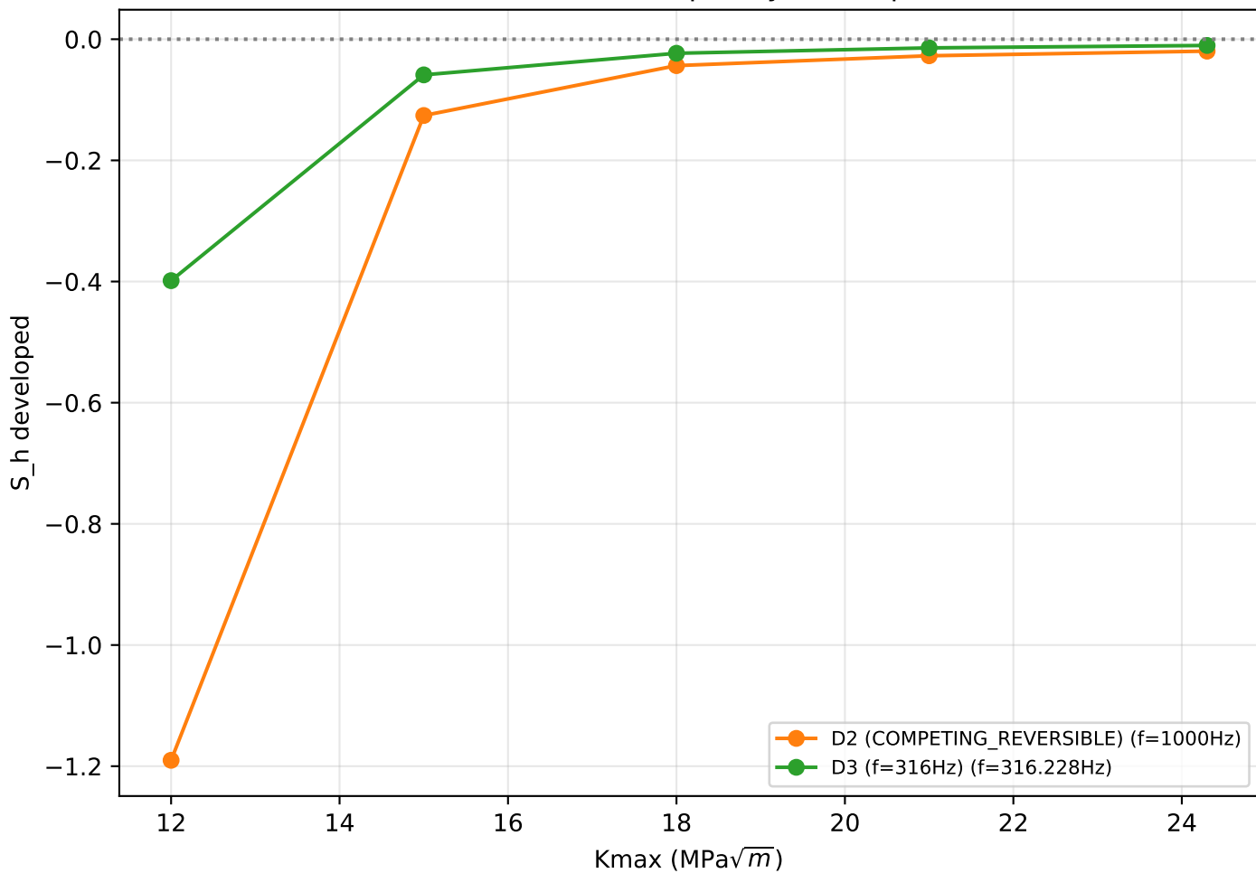
PHYSICAL SIMULATION: reduced-frequency developed curves (D2 vs D3)
