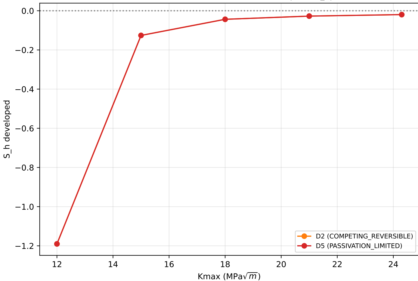
PHYSICAL SIMULATION: clean reversible (D2) vs passivation-limited (D5) developed curves (nearly indistinguishable -- \max|\Delta S_h|=0.0001 )
