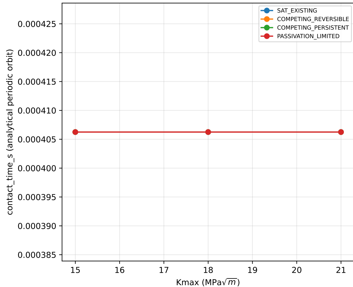
ANALYTICAL PREDICTION: available mechanism diagnostics vs Kmax (PX2 atlas grid: 15/18/21 MPa \sqrt{m} )
