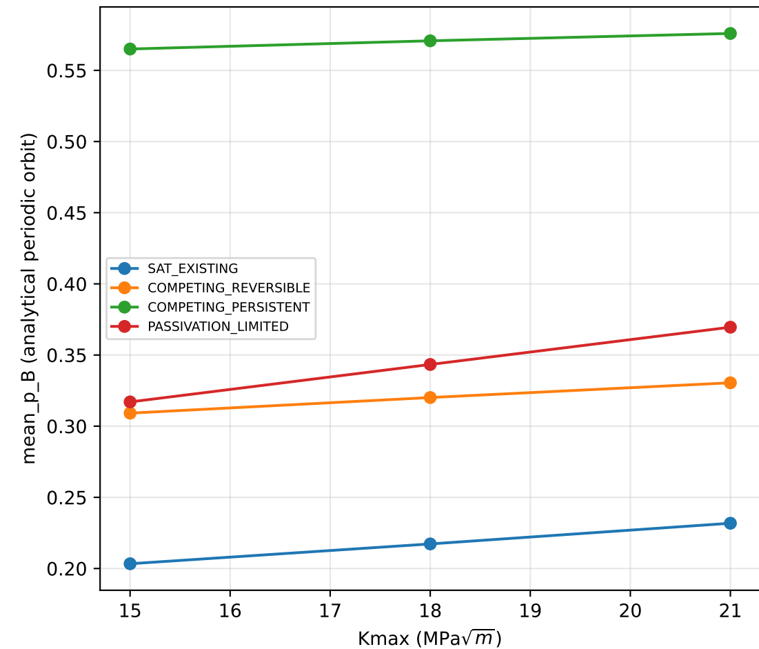
ANALYTICAL PREDICTION: available mechanism diagnostics vs Kmax (PX2 atlas grid: 15/18/21 MPa \sqrt{m} )
