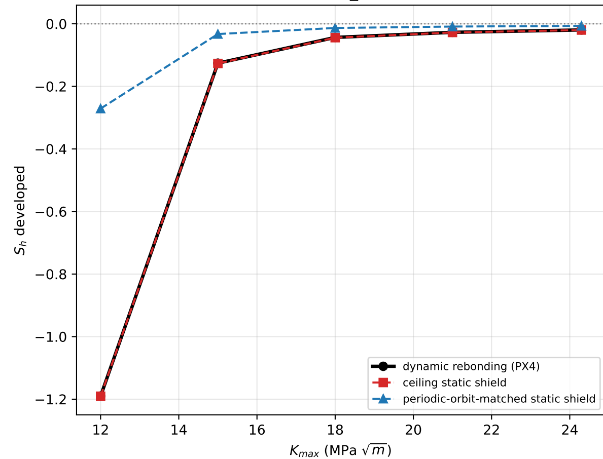
D2 (COMPETING_REVERSIBLE)
