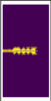
ceramic_V2_P25, 1200 K 1000.0 \mu\text{m} , REACHED_1000UM, step 1345
