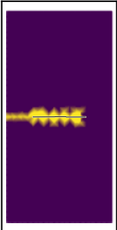
weakT_V2_P40, 1200 K 1000.0 \mu\text{m} , REACHED_1000UM, step 1345
