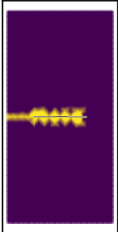
weakT_V2_P25, 300 K 1000.0 \mu\text{m} , REACHED_1000UM, step 2131
