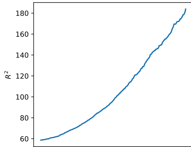
C3 at 900 K — 5 realizations
