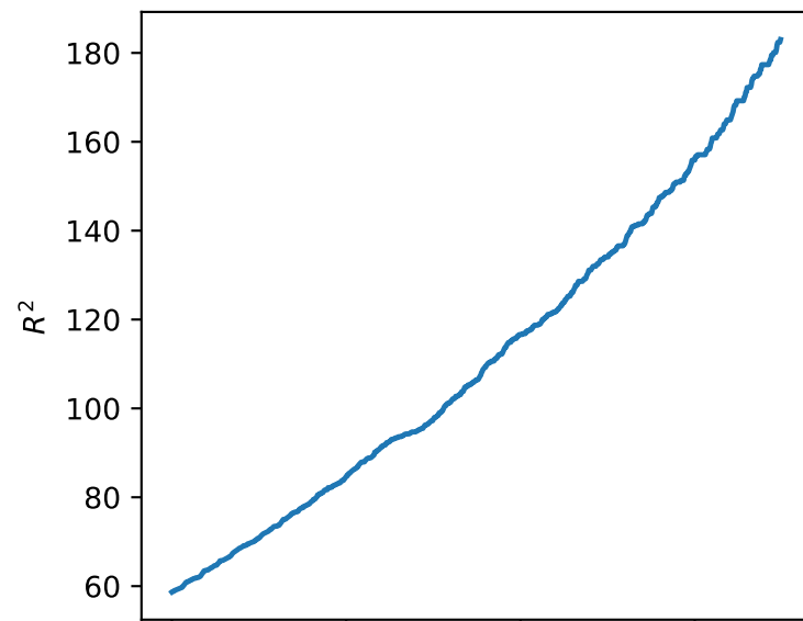
C4 at 900 K — 5 realizations
