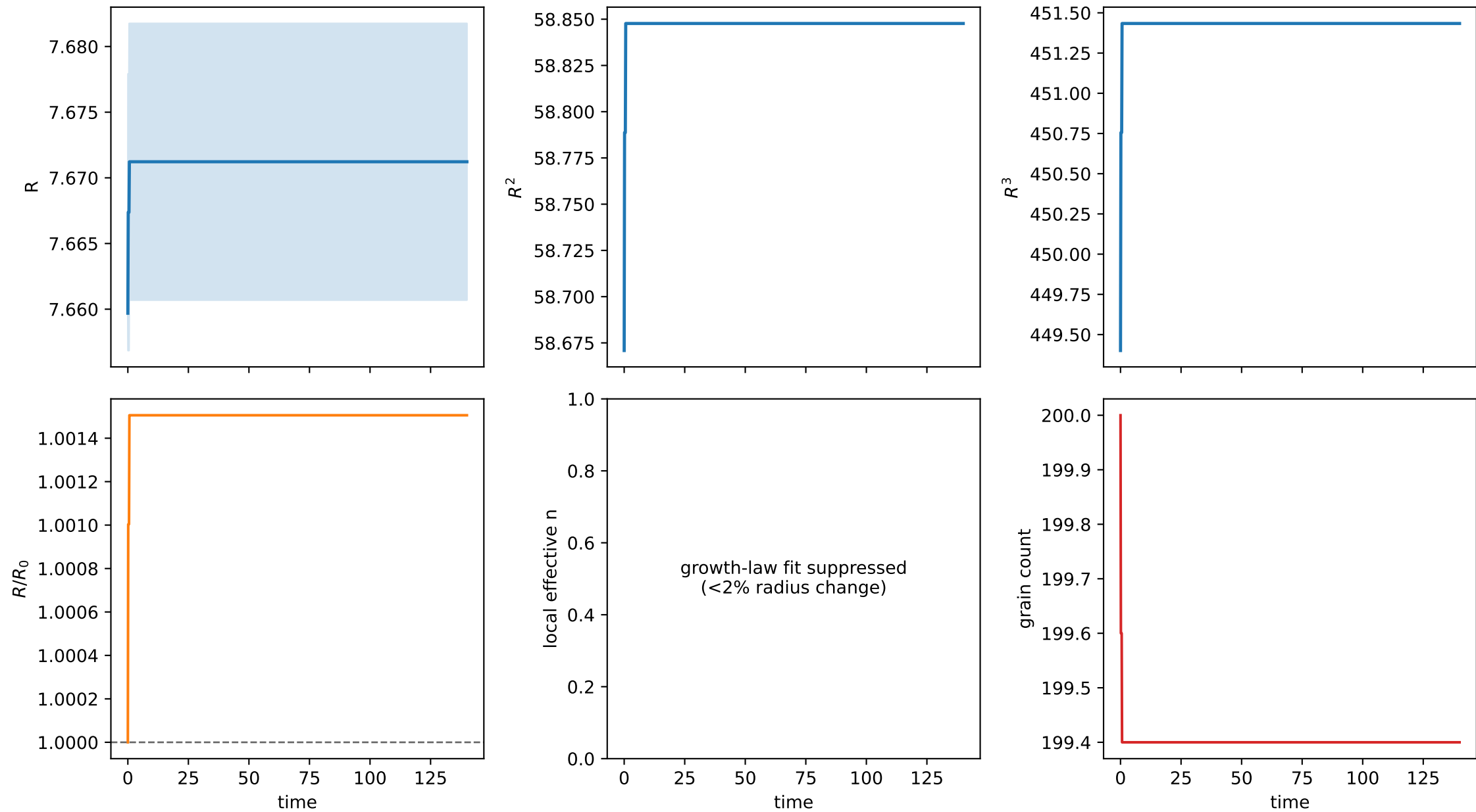
J2 at 900 K — 5 realizations
