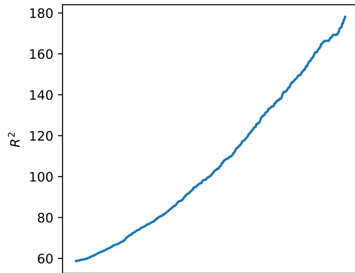
C2 at 900 K — 5 realizations
