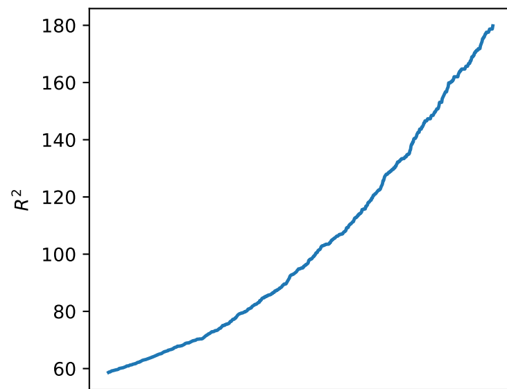
G2 at 900 K — 5 realizations
