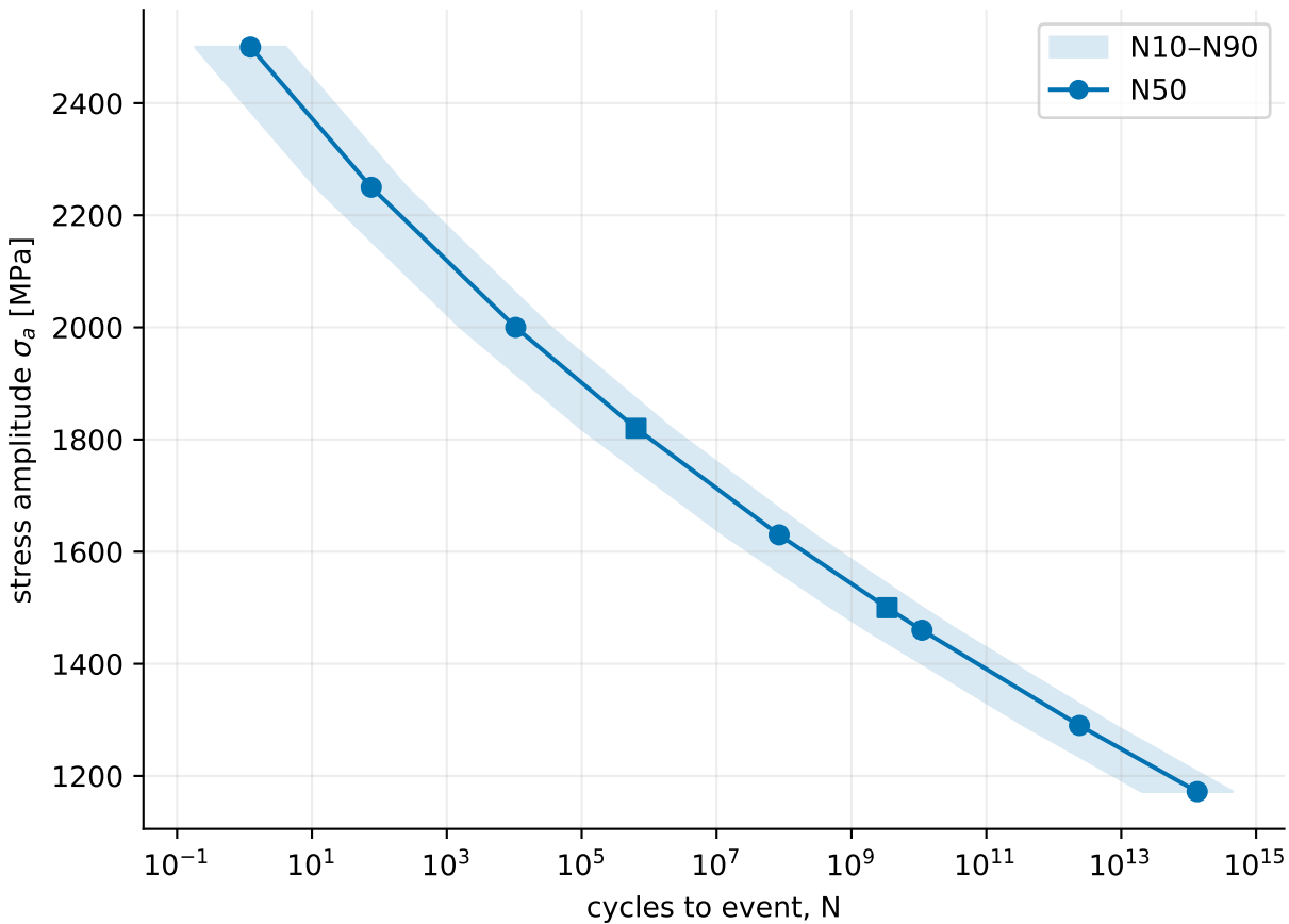
Peak Elementary-Attempt S-N Response 300 K, R=0.1, 1000 Hz; 600 \mu\text{m} blunt notch; one 10 \mu\text{m} segment
