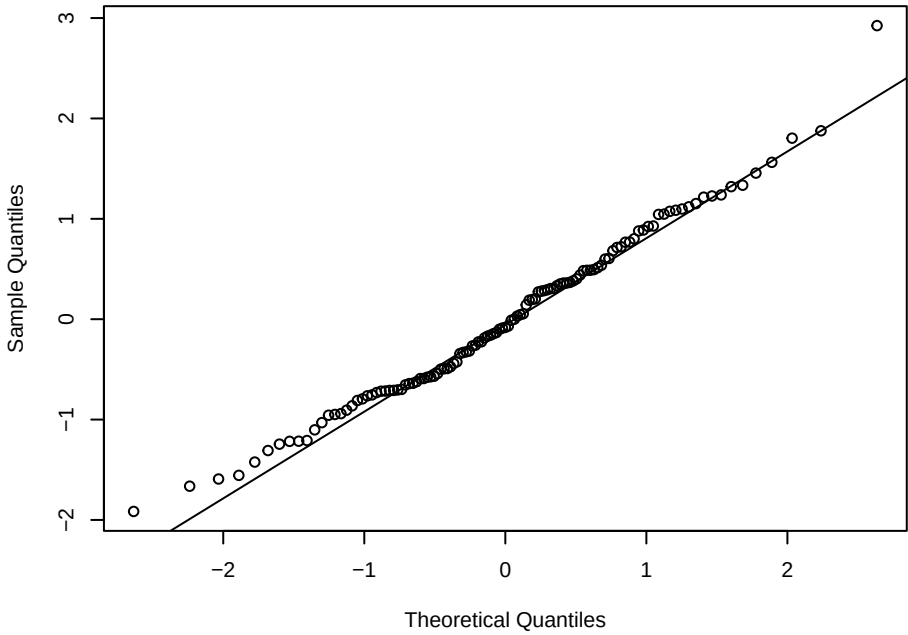
H2O – normal Q-Q
