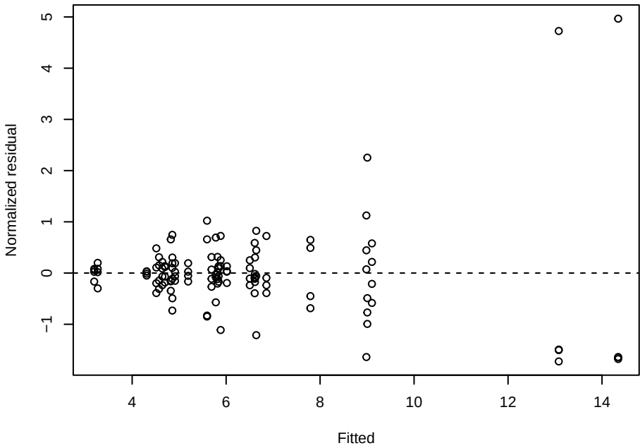
NH3 – residuals vs fitted
