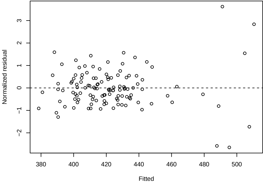
CO2 – residuals vs fitted
