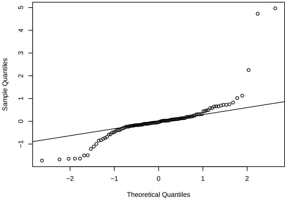
NH3 – normal Q-Q
