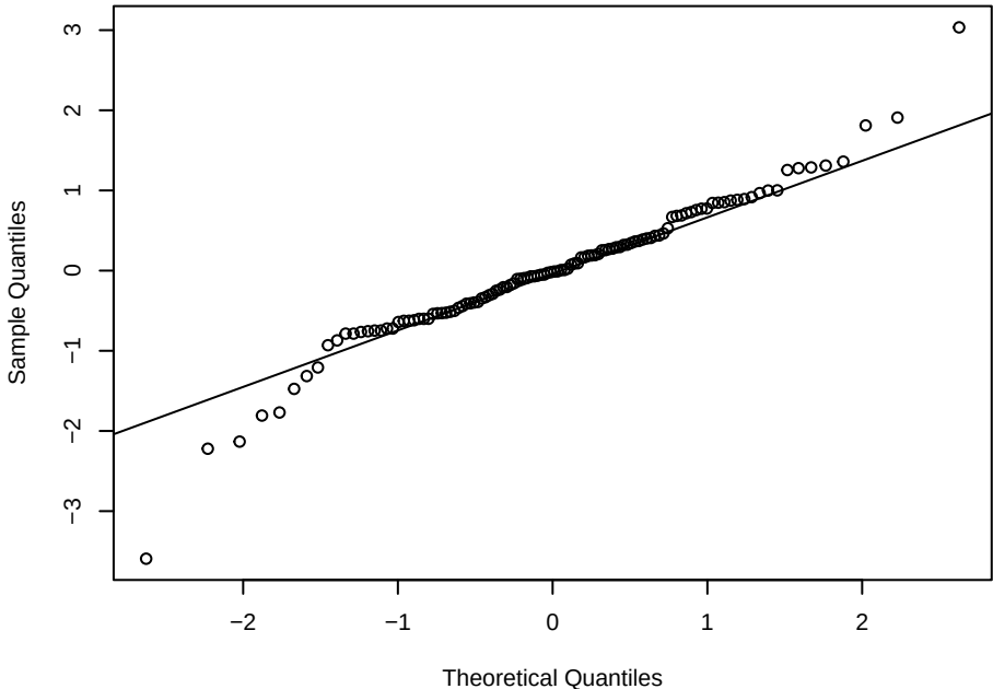
N2O – normal Q-Q
