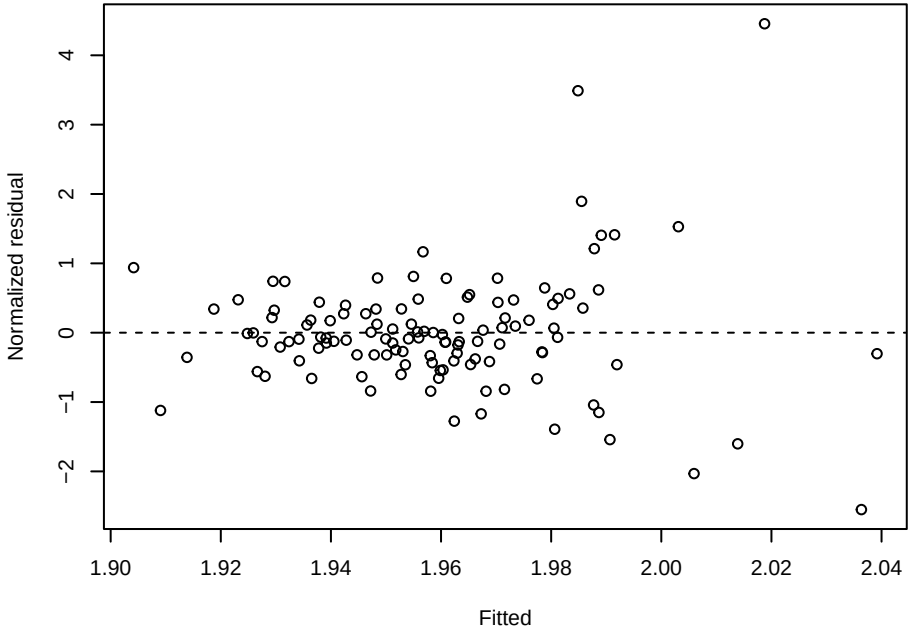
CH4 – residuals vs fitted
