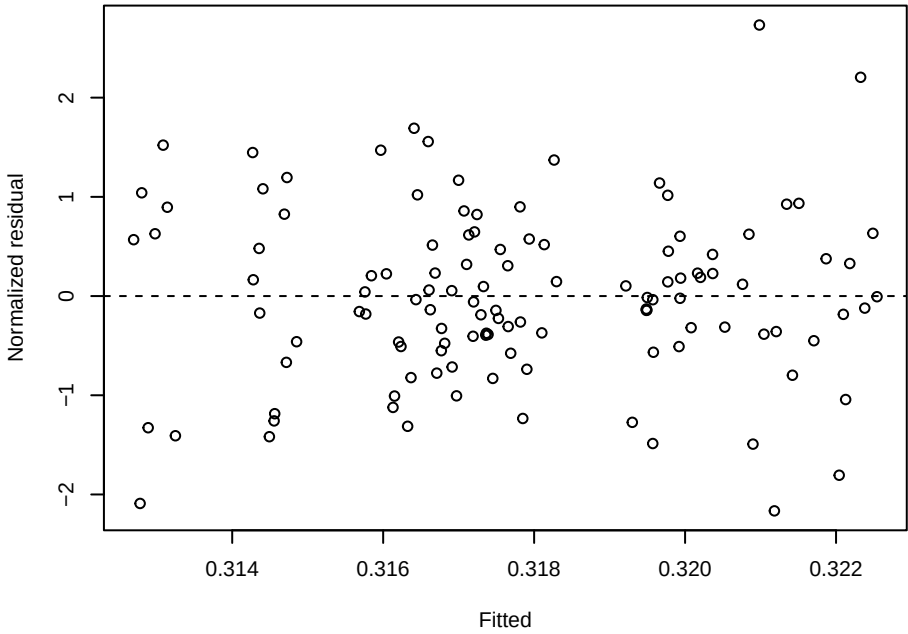
N2O – residuals vs fitted
