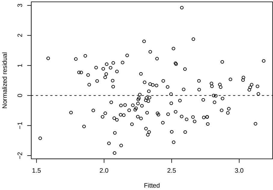
H2O – residuals vs fitted
