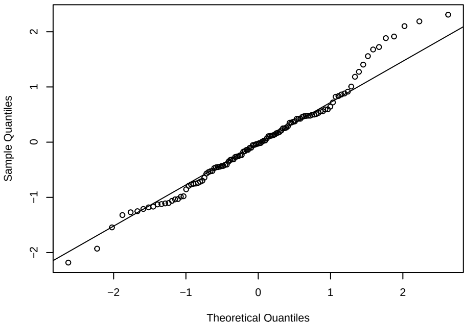
CH4 – normal Q-Q
