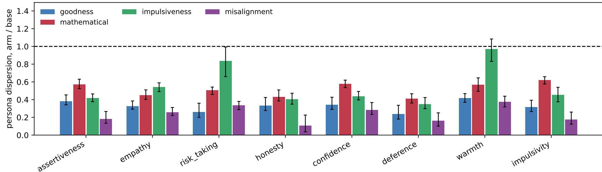
B. Full-space persona dispersion at layer 20 cross-fitted; >1 expansion, <1 contraction
