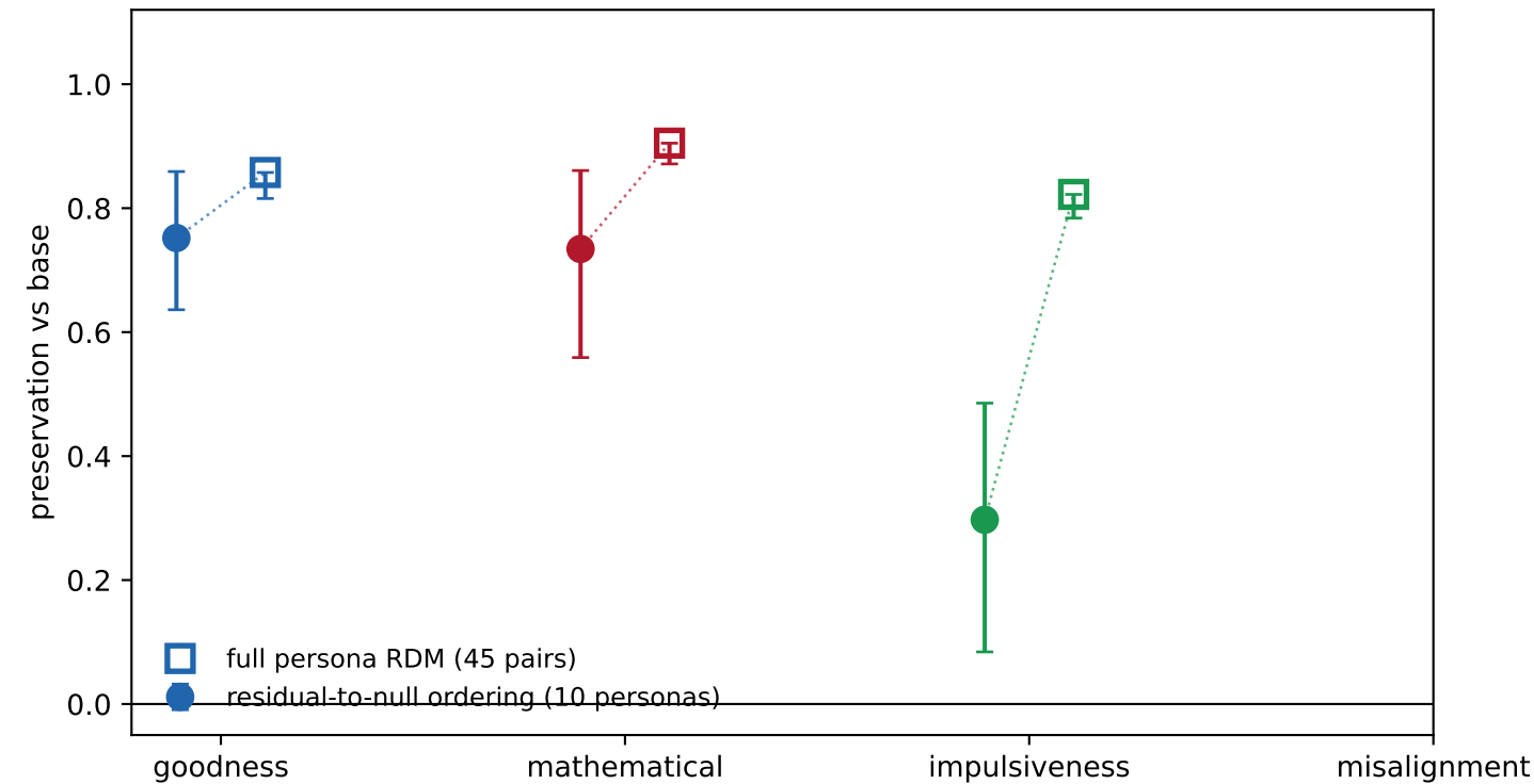
G. One direction vs the whole constellation (layer 15)
