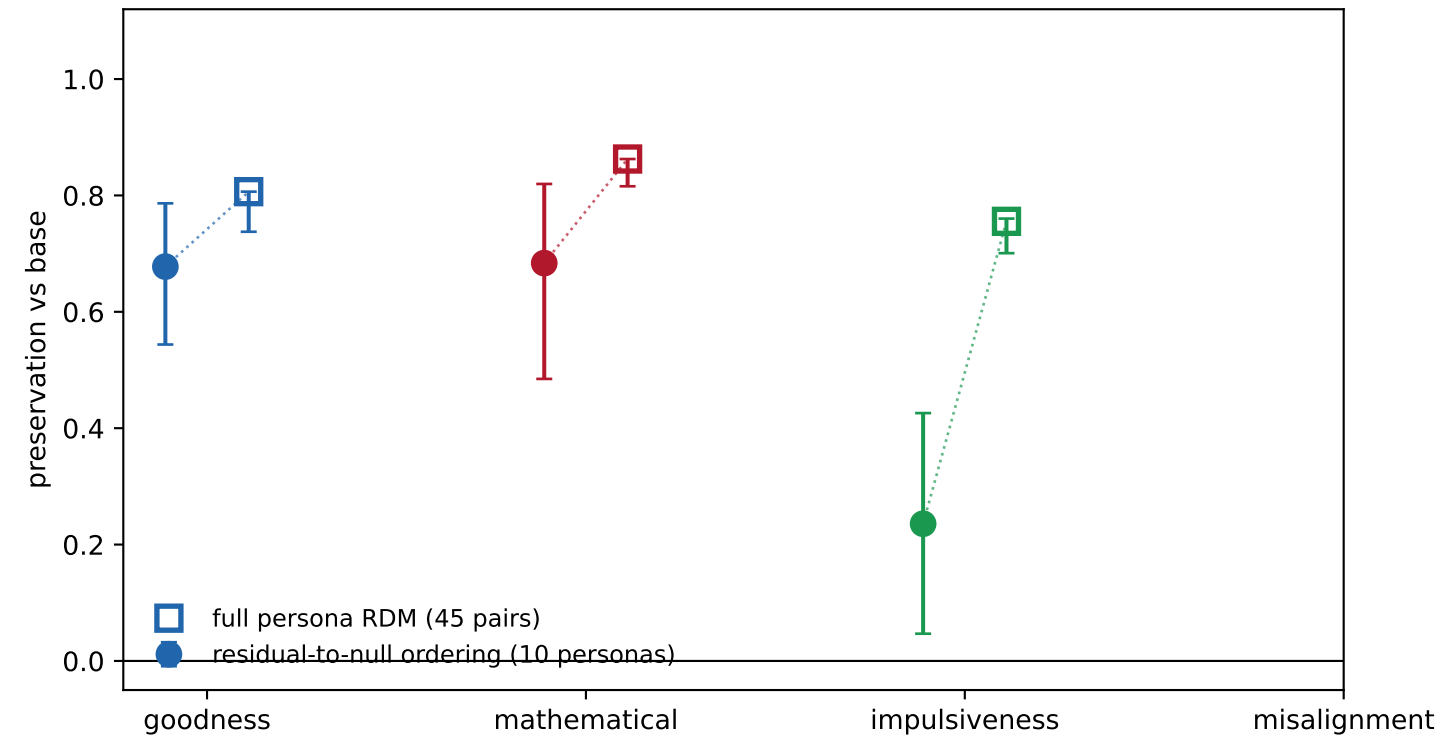
G. One direction vs the whole constellation (layer 20)
