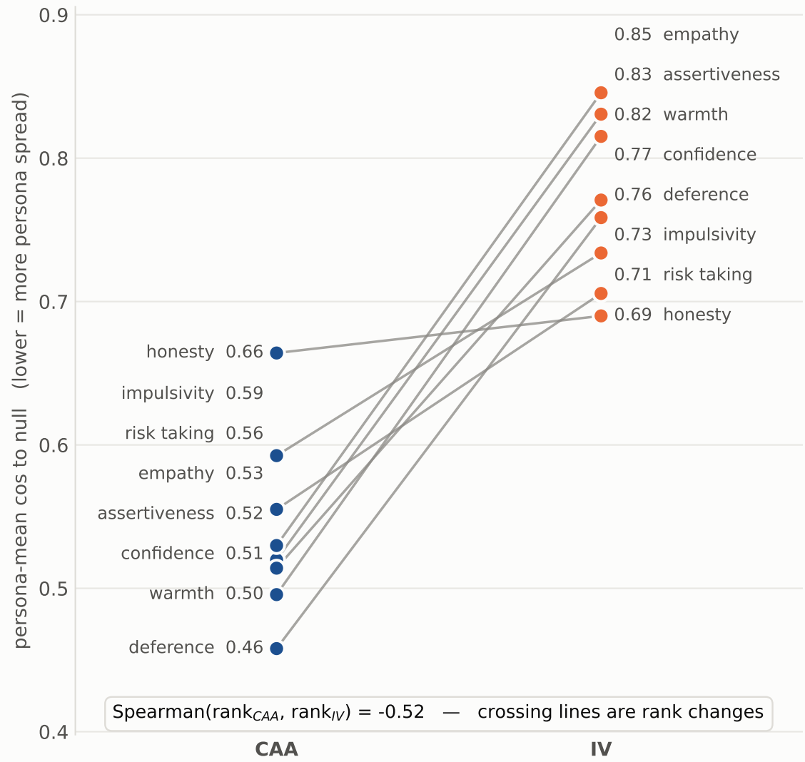
A. Same traits, two methods — layer 20
