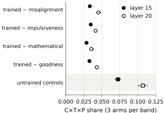
B CxT×P against an untrained reference
