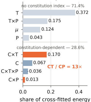
A variance partition (trained, L15)
