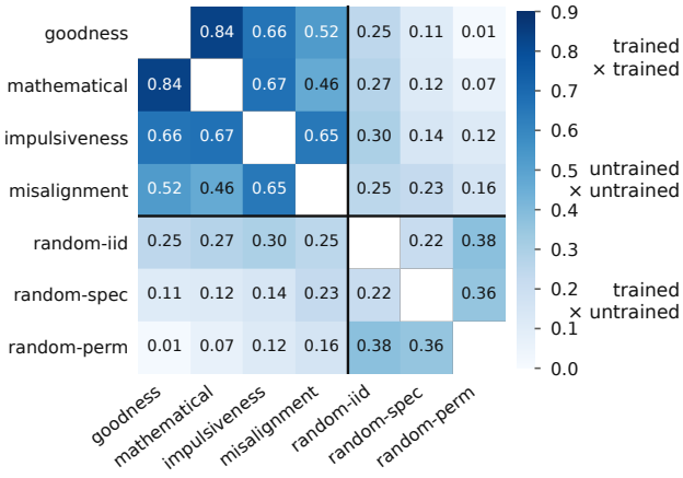
A \cos(dG, dG') at s = 1 , mean over 8 traits
