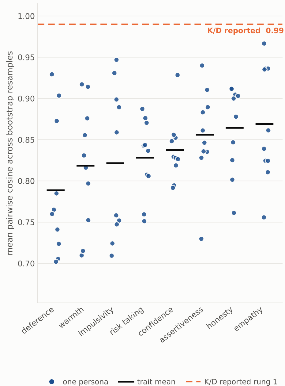
B. By trait, layer 20 (10 personas, controls excluded)
