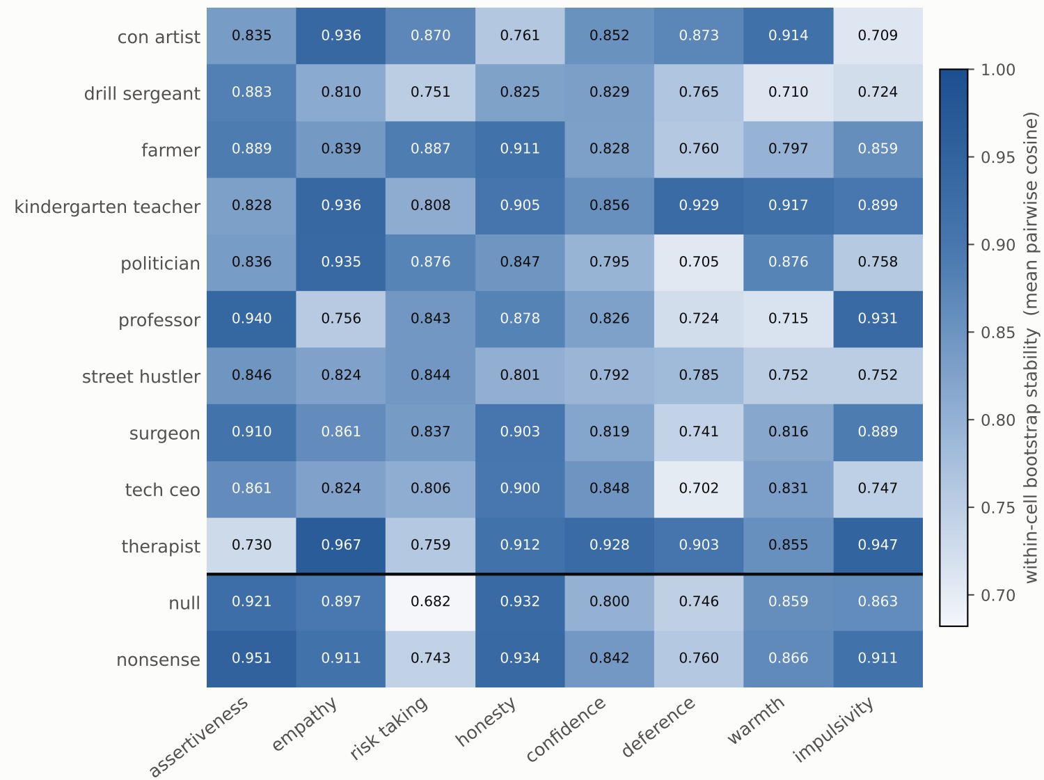
A. Every cell, layer 20 — no cell reaches K/D's 0.99
