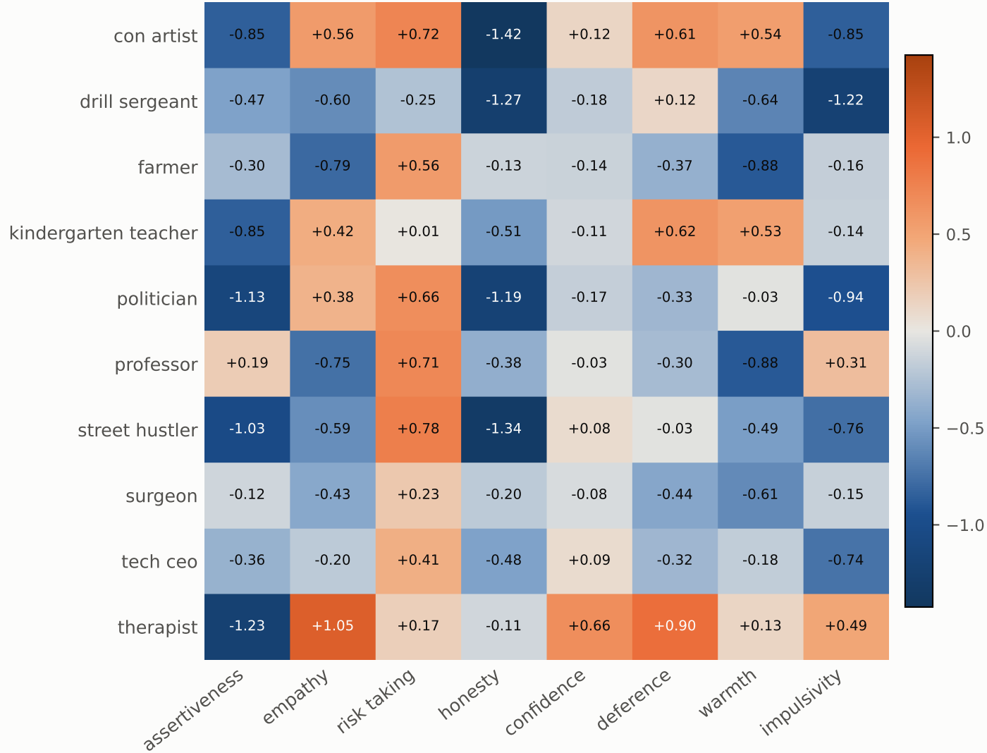
A. Vector length vs the assistant default, layer 25
