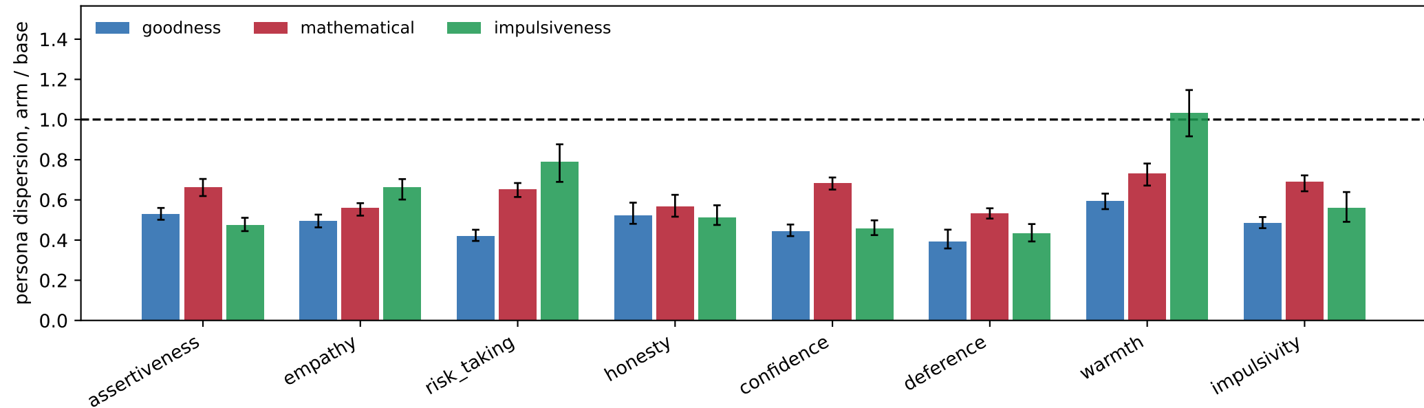
B. Full-space persona dispersion at layer 15 cross-fitted; >1 expansion, <1 contraction
