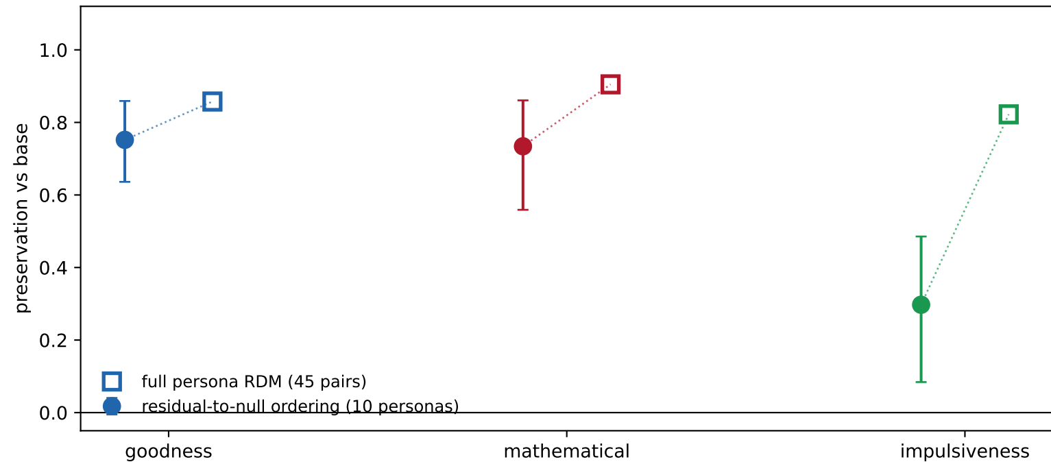
G. One direction vs the whole constellation (layer 15) filled = scalar ordering to the default direction; open = full persona RDM
