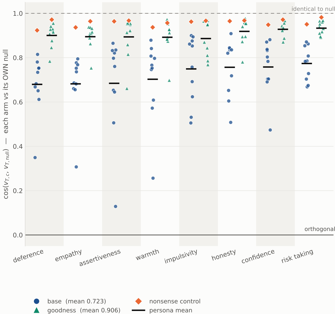
A. Persona spread under each arm (layer 15)
