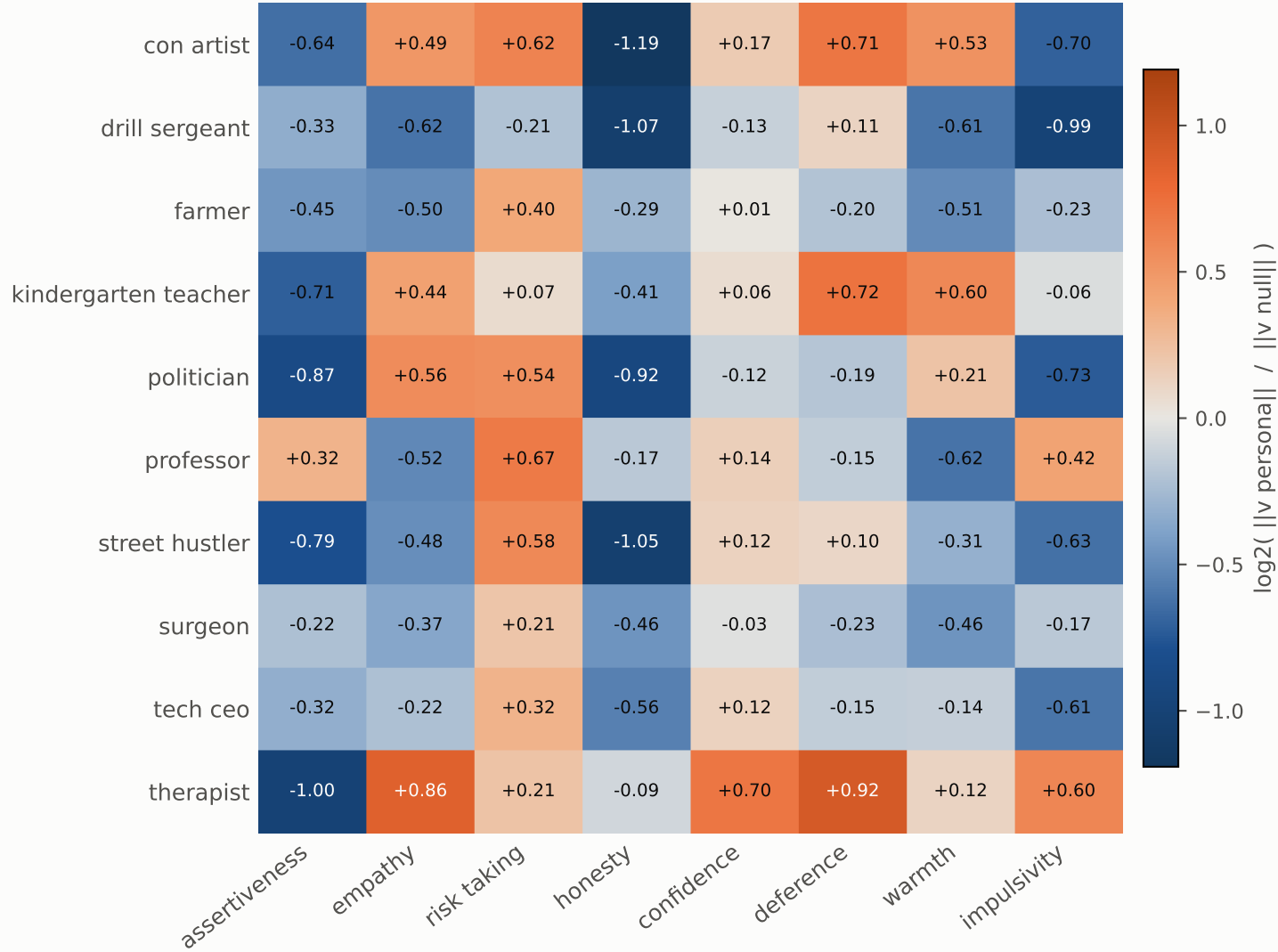
A. Vector length vs the assistant default, layer 20
