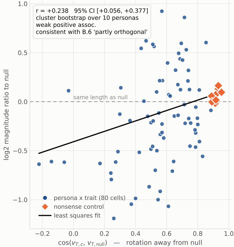
B. B.6 cell-level check, layer 20
