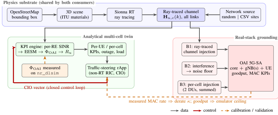
Fig. 1. System architecture. One physics substrate produces the ray-traced channel for every cell–UE link; two consumers share it. In the analytical twin, \Phi_{\text{OAI}} grounds throughput and the rApp closes a CIO loop. In the real-stack layer, three bridges drive a live OAI 5G Standalone system: comparing the twin against what OAI’s MAC schedules yields the constant derate \kappa , while comparing against delivered goodput additionally exposes the emulator’s ceiling.
